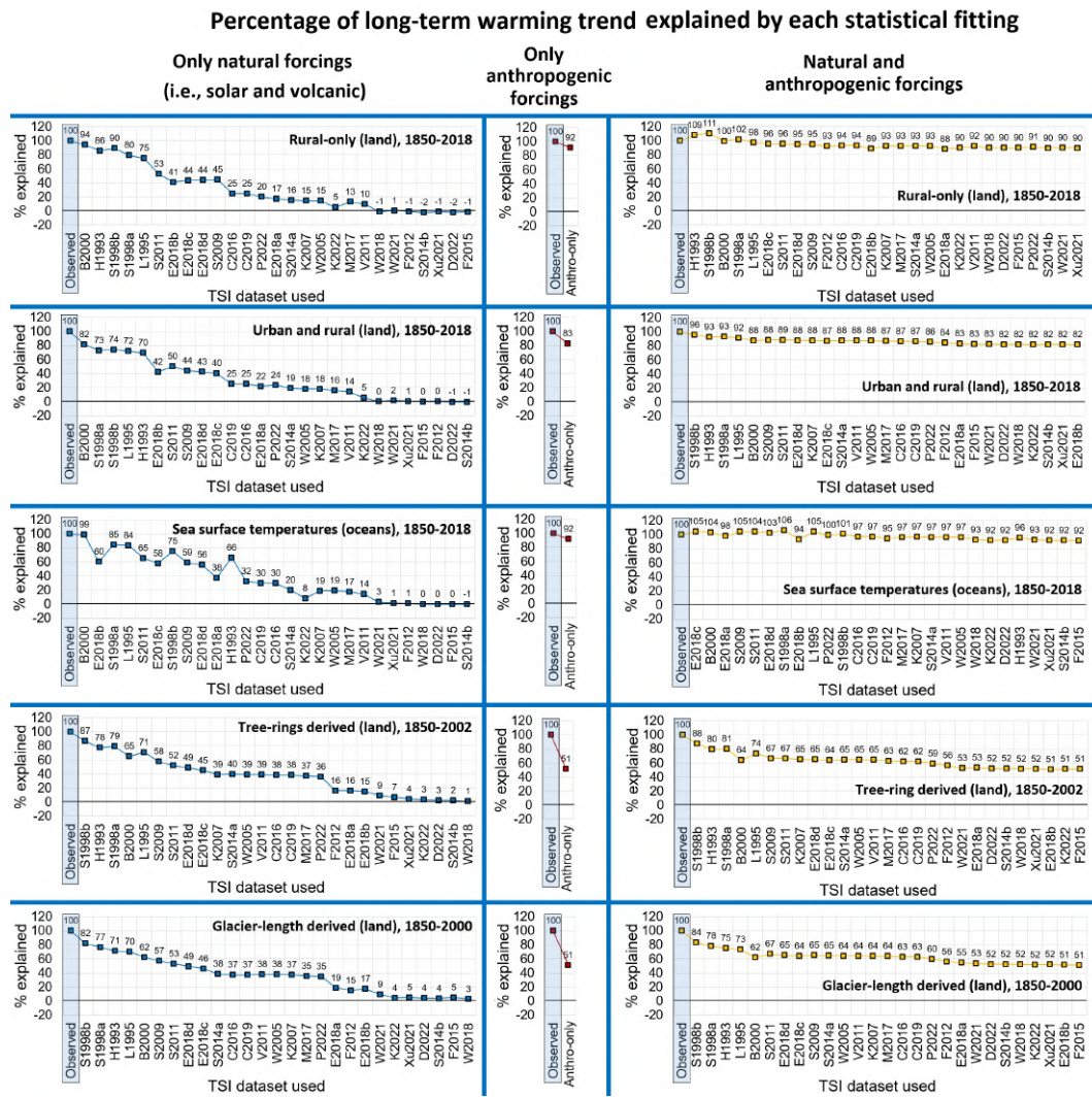
Fig. 5: Percentages of the long-term warming linear trend for all multi-linear regression fittings to each of the temperature series. The linear trends were calculated over the maximum overlap period: 1850–2018 for the three instrumental estimates; 1850–2002 for the tree-ring based proxies; 1850–2000 for the glacier-length based proxies. As for Figure 4, left hand panels correspond to the fittings using only natural forcings (solar and volcanic) with the results for each TSI dataset ranked as in Figure 4, i.e., from best fit (left) to worst fit (right). Middle panels show the results using only the anthropogenic forcings series. Right hand panels correspond to the combined “natural and anthropogenic” fits. Each row corresponds to a different ST record – from top to bottom: rural-only; urban and rural; sea surface temperatures; tree-ring based; glacier-length based.
