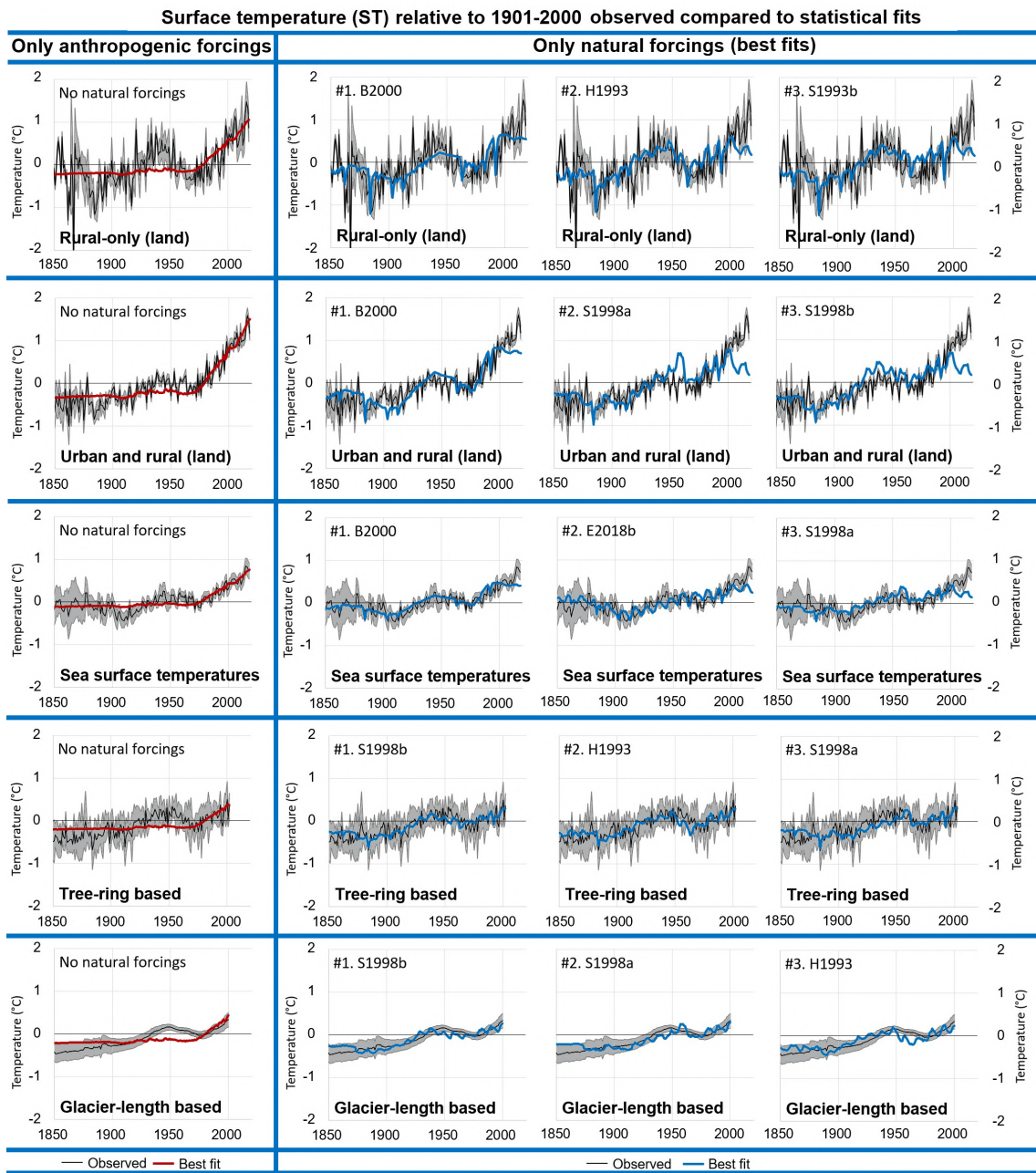
Fig. 6: Comparison of the various ST estimates (thin black line for mean estimates; gray envelope for associated uncertainty bands) to some of the statistical fittings. The left-hand panels correspond to the best fits using only anthropogenic forcings (thick red line). The other panels correspond to the three best statistical fits (in terms of r^2 ) using only natural forcings (thick blue line). Each row corresponds to a different ST record – from top to bottom: rural-only; urban and rural; sea surface temperatures; tree-ring based; glacier-length based.
